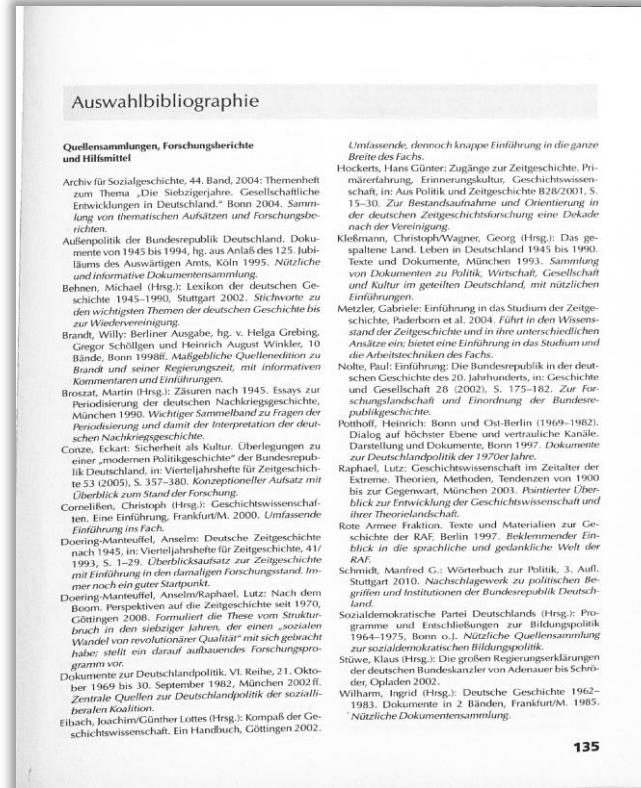
RGB Image
