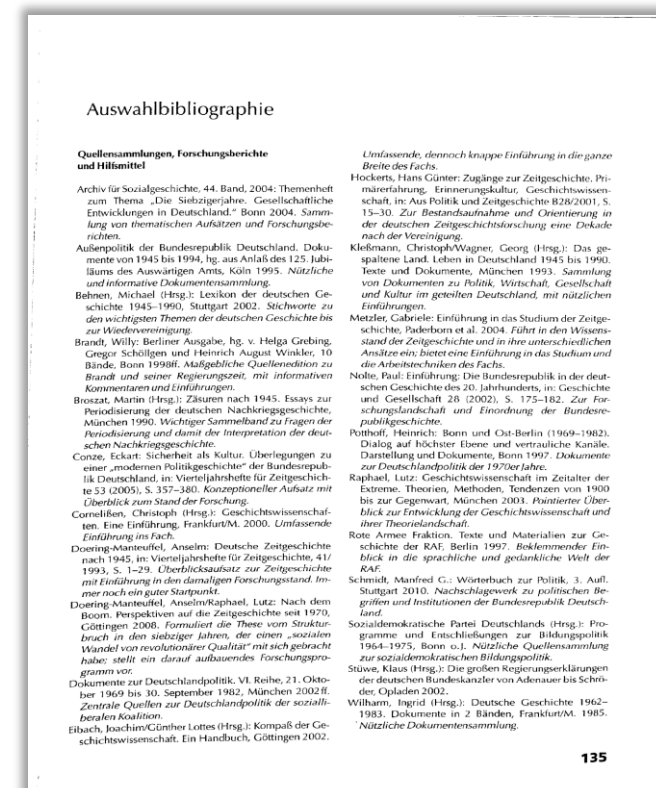
Binary Image
